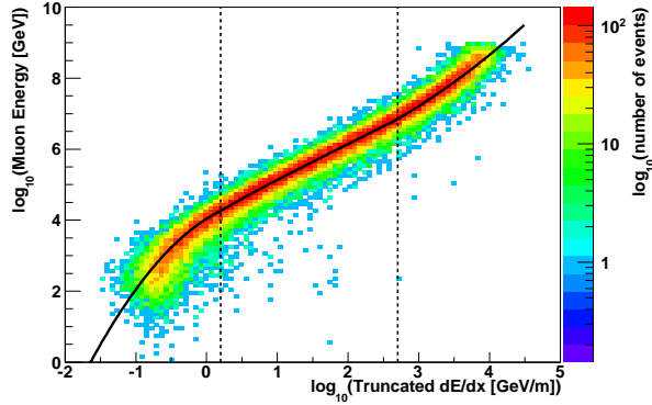
Figure 4: (color online) Simulated E_\mu vs. truncated dE/dx at the center of the detector, for the optimized 40% truncation. The distribution is much narrower than in Fig. 1. The vertical dashed lines identify the ranges for the three fit equations (represented by the solid black line).
