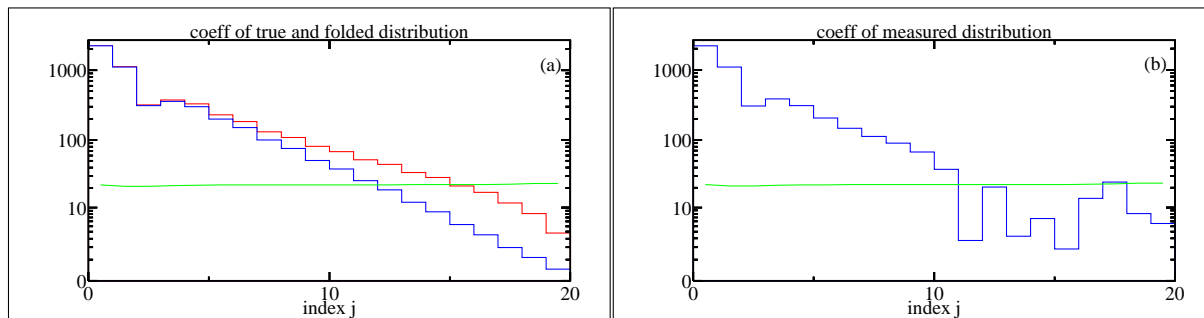
Fig. 3: The absolute values of coefficients b_j and c_j are shown for j = 1, 2, \dots, 20 . The coefficients b_j and c_j for the true distribution and the folded distribution (without measurement errors) are shown in (a), together with the (almost constant) error estimate for the coefficients b_j calculated by error propagation. The coefficients c_j from the simulated measured distribution are shown in (b), together with the error estimate. For j above 12 the smaller coefficients of the folded distribution become smaller than the statistical error. In (b) the coefficients for j above 12 are dominated by statistical errors and even the sign is not determined by the data.
