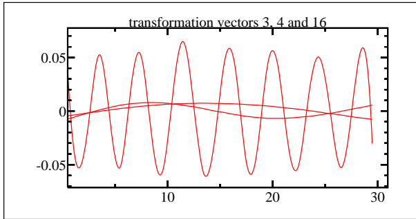
Fig. 4: Selected column vectors of the complete transformation matrix defined in the regularization procedure. They correspond to the curvature eigenvalues S_{33} , S_{44} and S_{16,16} . Visualization is done by curves interpolating the components. The amplitude associated with each vector all have the same standard deviation of 1.
