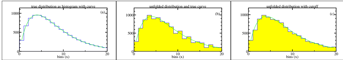
Fig. 2: Original (true) distribution (a) and two results from unfolding ((b) and (c)). Result (b) has been obtained from all 20 coefficients, and for result (c) a sharp cut-off after 10 coefficients has been applied (i.e. the coefficients 11 to 20 are ignored).
