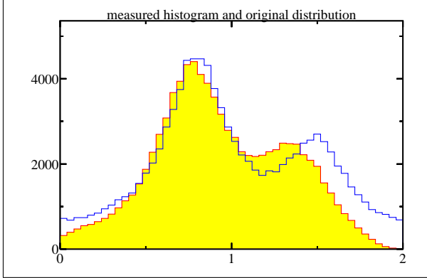
Fig. 1: The Monte Carlo simulation of the effects of limited acceptance, transformation and finite resolution. Shown is the original (true) distribution (line histogram) and the "measured" distribution (yellow/shaded histogram).
