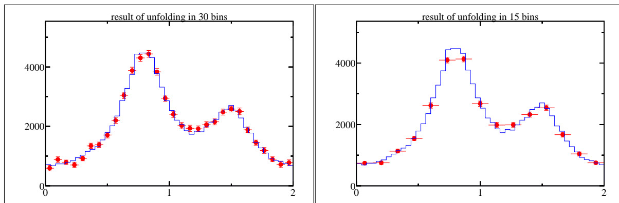
Fig. 6: The unfolding result after regularization with 15 degrees of freedom with 30 bins (left) and with 15 bins (right). For comparison the original (true) distribution is shown by a histogram. The data from Figure 1 are used as input.
