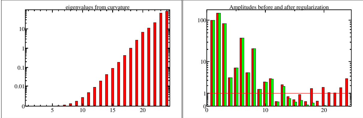
Fig. 5: The eigenvalues after the curvature transformation. The values are very rapidly increasing for orthogonal contributions for increasing index value (left). The amplitudes before (left bars) and after regularization (right bars). The statistical error of all amplitudes is equal to 1, which is indicated by the horizontal line. The vertical scale is linear at the bottom and makes a transition to a logarithmic scale at the top (right).
