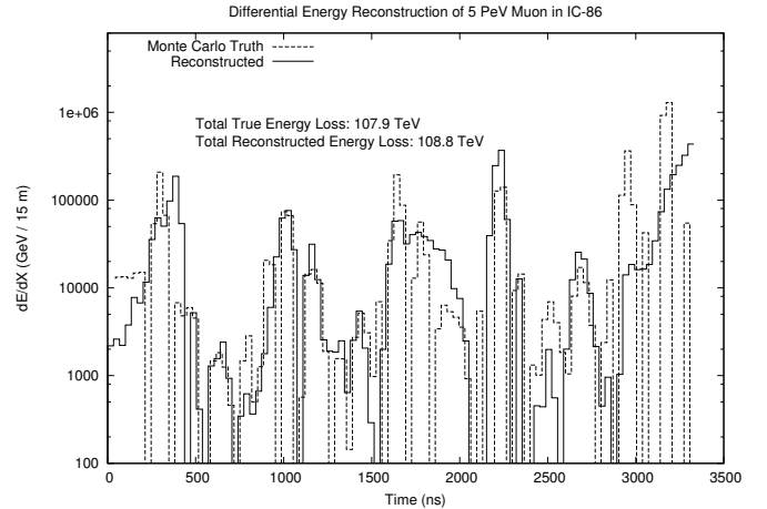
Figure 17: Reconstruction of the energy deposition of a simulated 5 PeV single muon using unfolding with a 15 meter cascade spacing. For this event, the total reconstructed energy loss within the detector differs from the true value by less than 1%.
