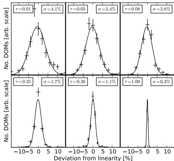
(b) Fractional deviations of observed light amplitudes from predictions, assuming a linear scaling, in 276 DOMs that triggered in response to calibration laser pulses at six different filter transmittance settings ( \tau in each panel). Each entry in each histogram is the proportional deviation of the collected charge from a best-fit line like those shown in (a). The linear fit effectively pivots around the highest transmittance setting (lower right panel). The largest deviations are at the lowest transmittance setting (upper left panel), and are on the scale of 5%.
