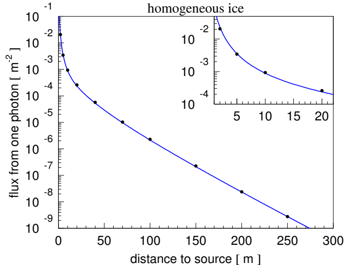
Figure 4: Approximations to the observed light level as a function of distance for point light sources. Lines show Eq. 5. Results from a Monte Carlo simulation of photon tracking are shown with black points. The insert at the top right shows small distances. These plots are made assuming homogeneous optical properties of the ice, whereas the actual glacial ice has depth-varying properties [18].
