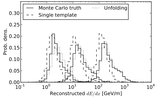
(b) Slices of the reconstructed energy loss rate distributions shown in (a) at fixed muon energies of 10^4 , 10^5 , and 10^6 GeV.
