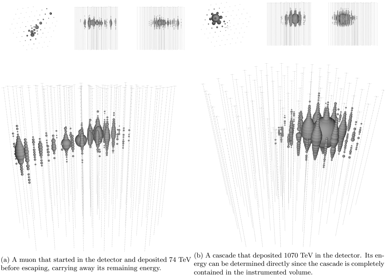
Figure 2: Examples of neutrino event topologies in IceCube from [12]. Each panel is a schematic view of the detector, with each photomultiplier represented by a sphere whose volume is proportional to the collected charge. The smaller upper panels show projections of the detector along its z , x , and y axes, respectively.
