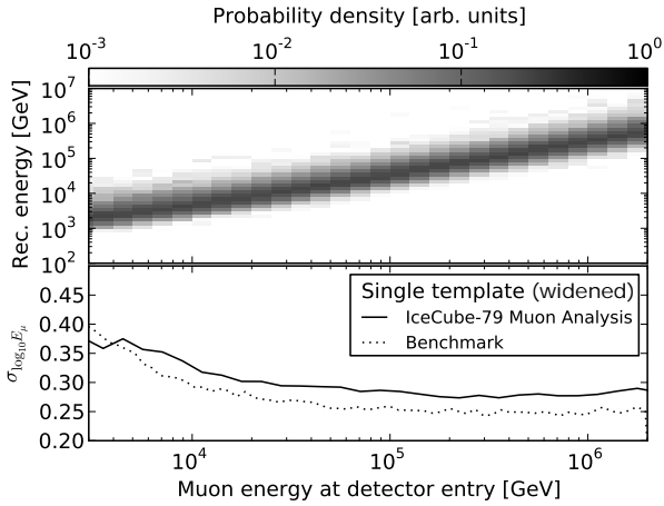
Figure 22: Energy resolution for a sample IceCube muon analysis at final level. The slight reduction in resolution at high energies compared to the “benchmark” level (from Fig. 21) arises from convolution of the intrinsic energy resolution (“benchmark”) with the finite resolution of the angular and positional reconstruction used in this analysis.
