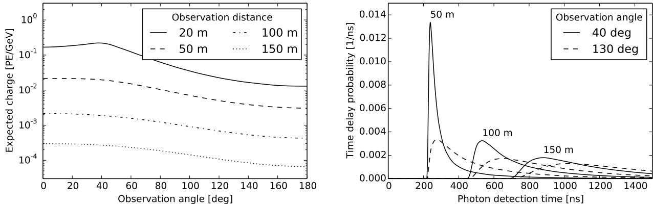
(a) Total observed light level as a function of radial distance from the source and observation angle with respect to the source direction. While scattering in the ice washes out the Cherenkov angle, the direction of the source remains visible as an asymmetry even at large distances. (b) Normalized time distribution of detected photons at different distances for two observation angles. Photons detected at the Cherenkov angle have generally experienced the least scattering, and so are detected earlier and more closely bunched in time than those detected at other angles.
