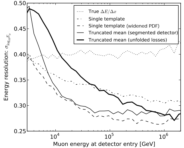
Figure 21: Comparison of the energy resolution of various methods on simulated through-going muons using the measure illustrated in Fig. 20. The true mean energy loss rate is shown for purposes of comparison only and provides a poor energy proxy no matter how precisely it can be reconstructed.
