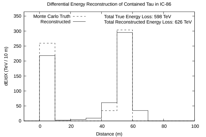
(b) Differential energy reconstruction showing two separated peaks, a distinct signature of \nu_\tau interactions. Detailed dE/dx reconstruction may allow identification of these interactions with decay lengths smaller than the scale of the detector instrumentation.
